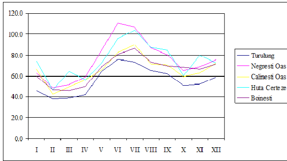
Fig. 2 The Chart of multi-annual monthly average rainfall (l/square meters)
