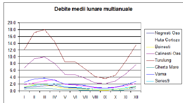
Fig. 4 Multi-annual monthly average flows ( m³/s)
